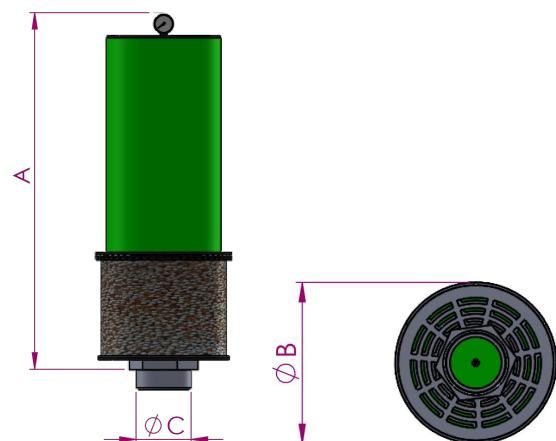
KH-1000 A: 710mm B: 272mm C: 4"
